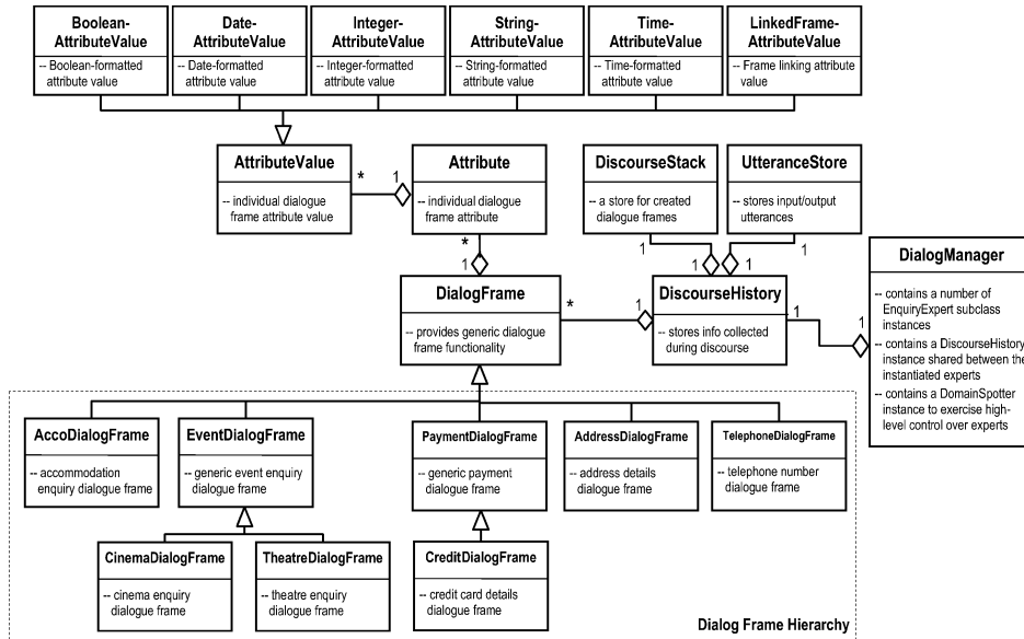
Fig. 2b. The Knowledge Hierarchy.
